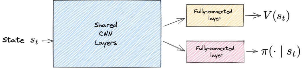
Figure 3: Example of a shared network architecture for actor-critic methods.
