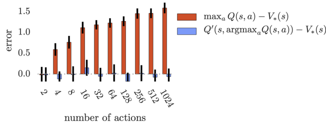
Figure 2: Red bars (resp. blue bars) show the bias in a single Q-learning update (resp. double Q learning update) when considering i.i.d. Gaussian noise. Figure taken from [10]
