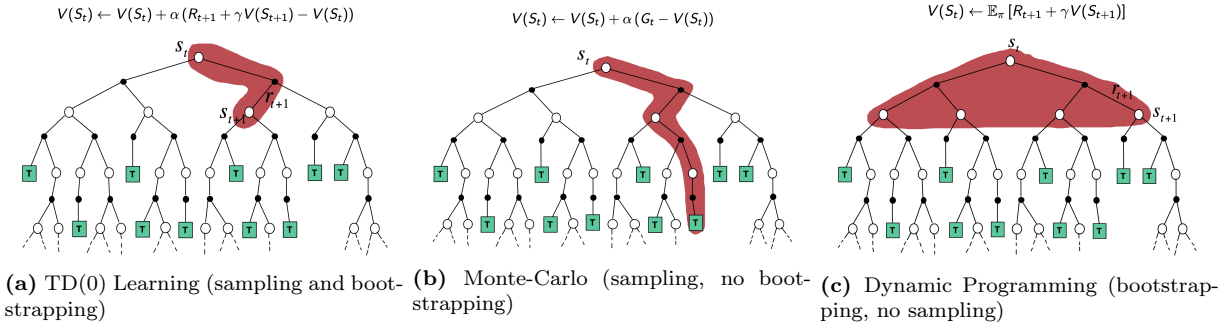
Figure 1: Different approaches to learning value functions. By using an estimate in the update, bootstrapping methods do not need to go as deep and can be faster, although they introduce bias. Unless the MDP is known, sampling is necessary. Figures taken from David Silver notes [1], lecture 4 on Model-Free prediction.
